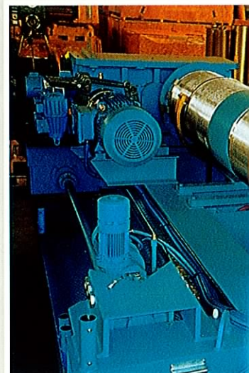
Carrello argano per gru a ponte - P Winch crab for bridge crane - Capa
